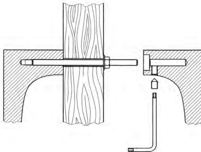
Montaje juego manillones Concealed back to back fixing assembly set of pull handles.
